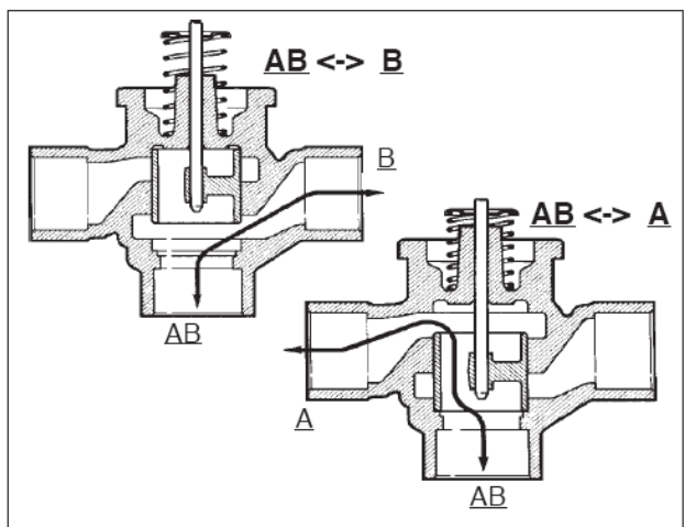
Fig. 2 - Fluid flow of 3-way valves
