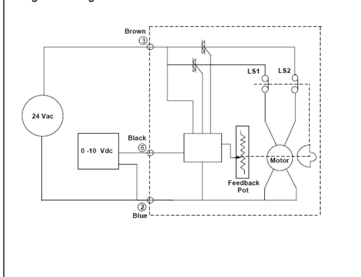
Fig. 8 - Wiring Schematic of the VC7900 Series Actuators
